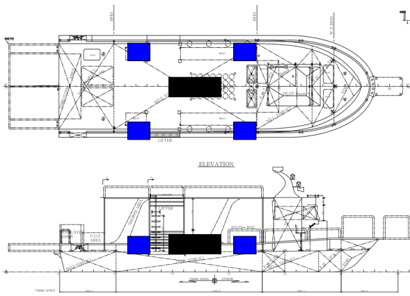
Fig. 8 GT 3.7 General Arrangement of AL Diving Boat (Opened flow type)
