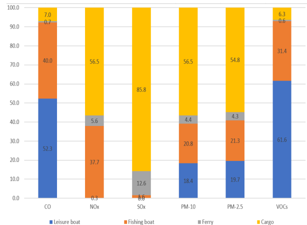
*출처: National Fine Dust Information Center, 2020. Statistics on air pollutant emissions Fig. 3. Ratio of total air pollutant emissions by ship type
