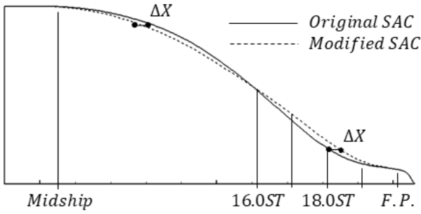
Fig. 1 SACs of fore body for the original and the modified hull form(Hull form variation by SAC)
