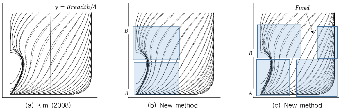
Fig. 24 Comparison of body plans (U-V type)
