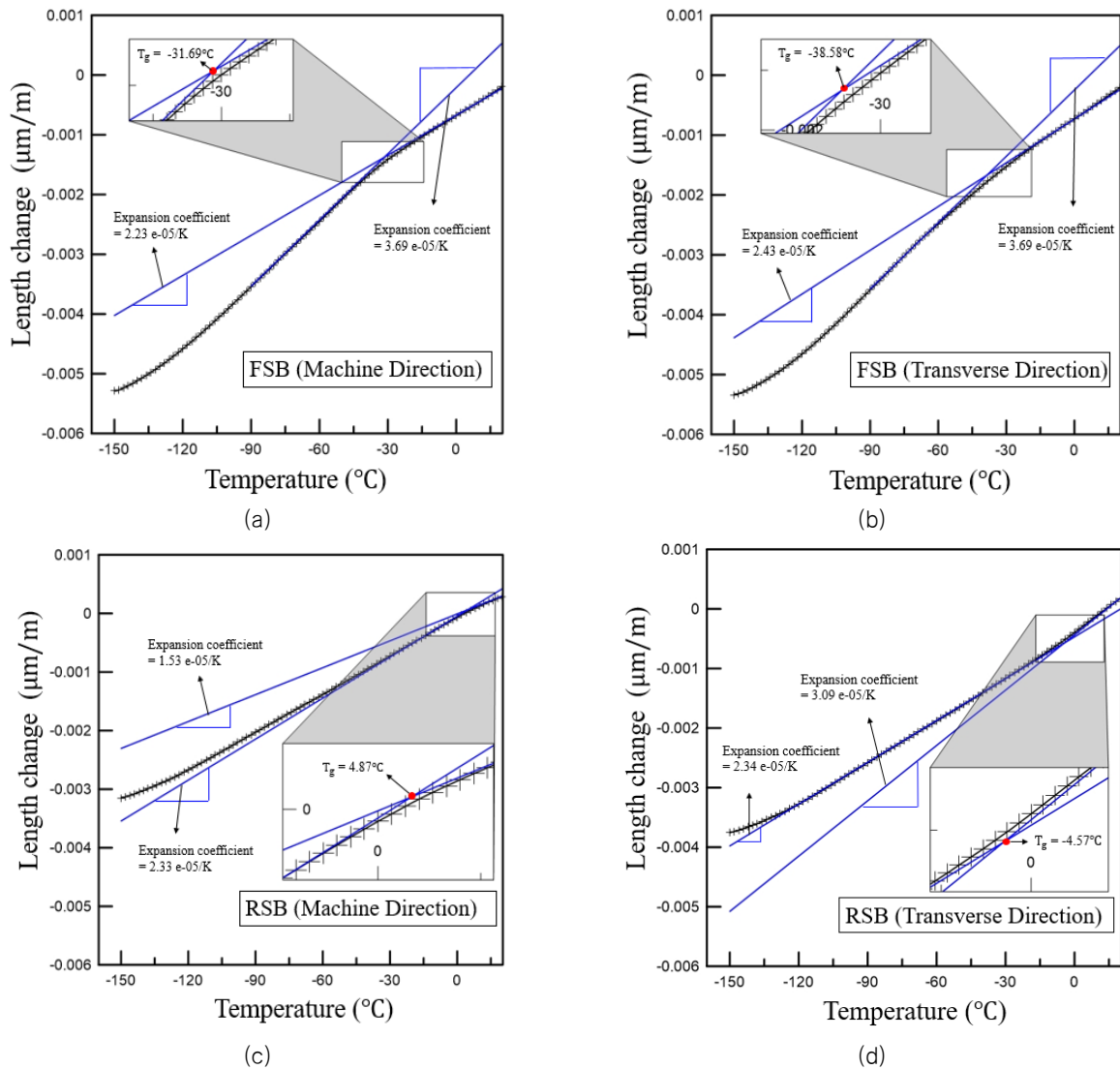
Fig. 5 Measure of Coefficient of Thermal Expansion(CTE) & glass transition temperature using Thermal Mechanical Analysis(TMA); (a) FSB(machine direction) (b) FSB(transverse direction) (c) RSB(machine direction) (d) RSB (transverse direction)
