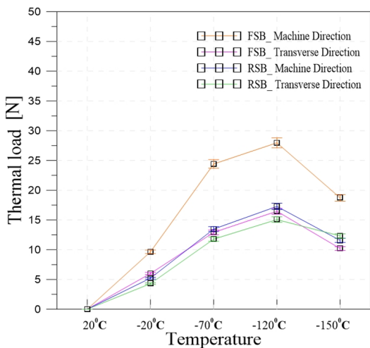
Fig. 9 Diagram of thermal load in secondary barrier
